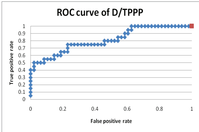
Figure 1: ROC curve for the D/TPPP ratio.
