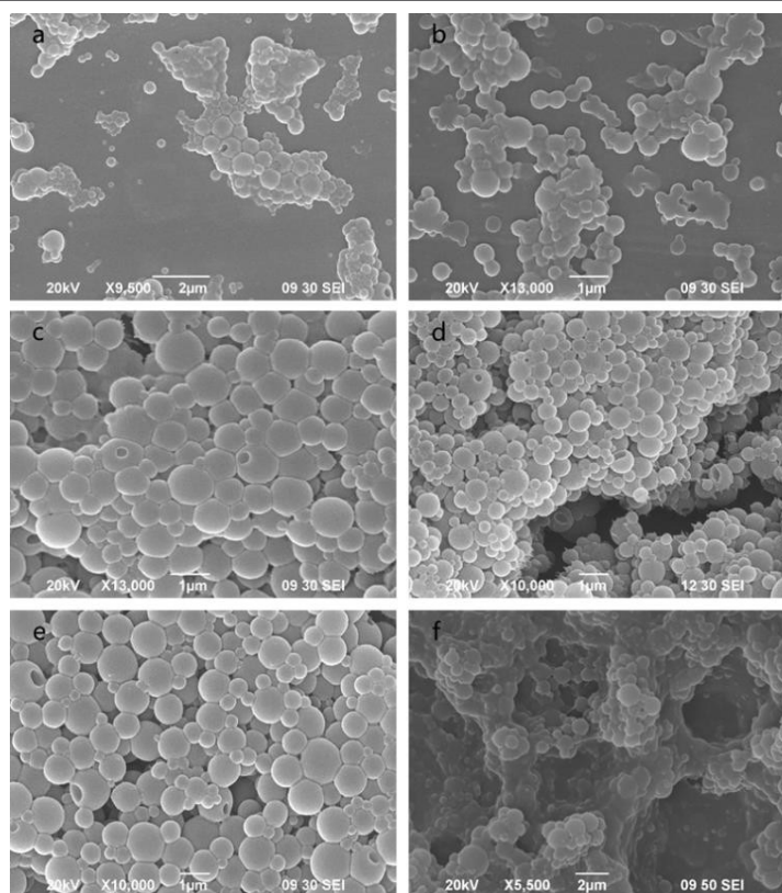
Figure 1: SEM images of VC-encapsulated zein/CS microspheres with different zein/CS mass ratio of (a) 0.5:1, (b) 1:1, (c) 1.5:1, (d) 2:1, (e) 2.5:1, and (f) 3:1.
