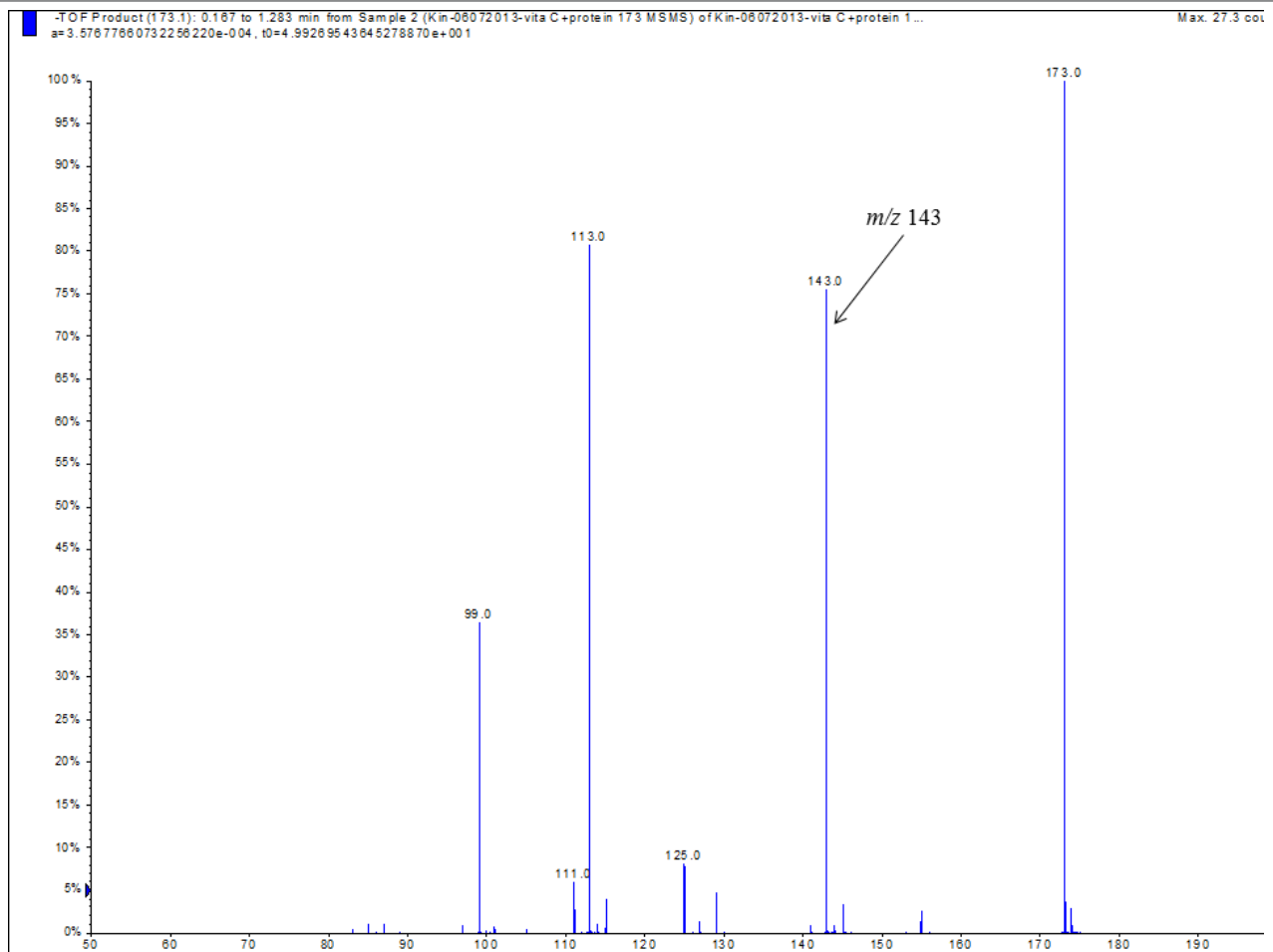
Figure 3: Negative ion ESI-MS/MS spectrum for the m/z 173 ion
