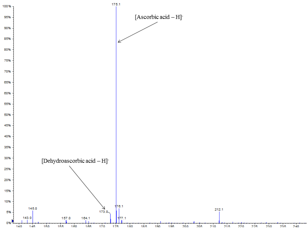
Figure 2: Negative ion ESI-MS spectrum for the VC-encapsulated zein/CS micro spheres.
