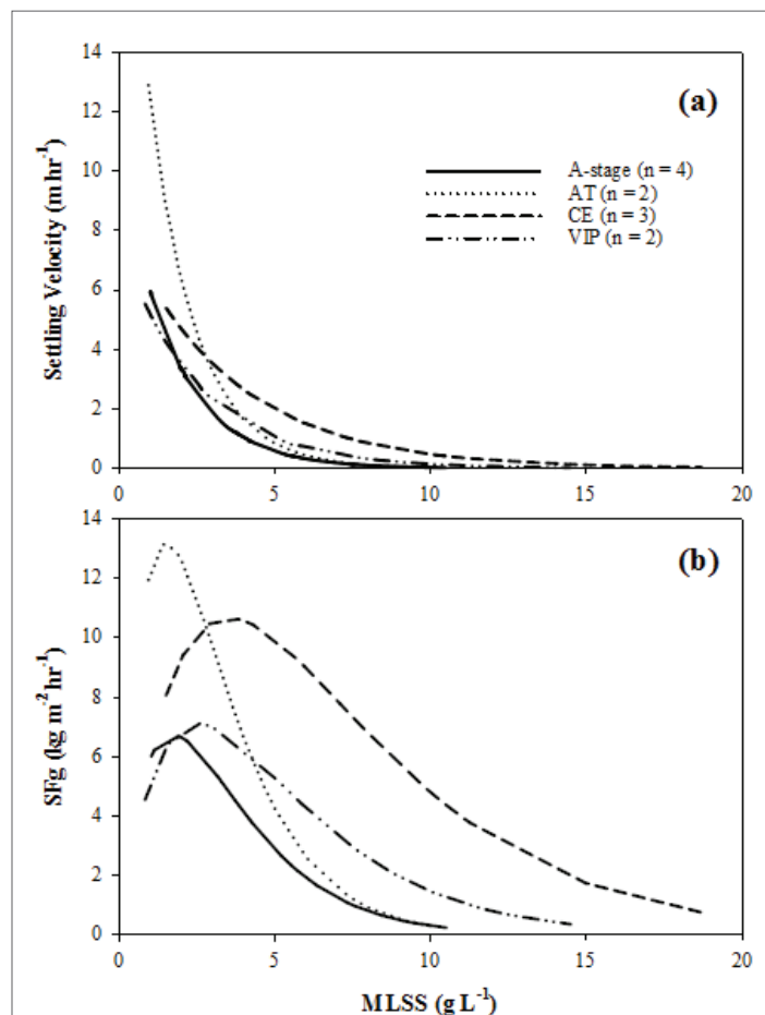
Figure 3: Comparison of (a) modeled settling velocity and (b) SFg to initial MLSS concentrations during ZSV tests on mixed liquor samples from the pilot A-stage and AT, CE, and VIP treatment facilities.
