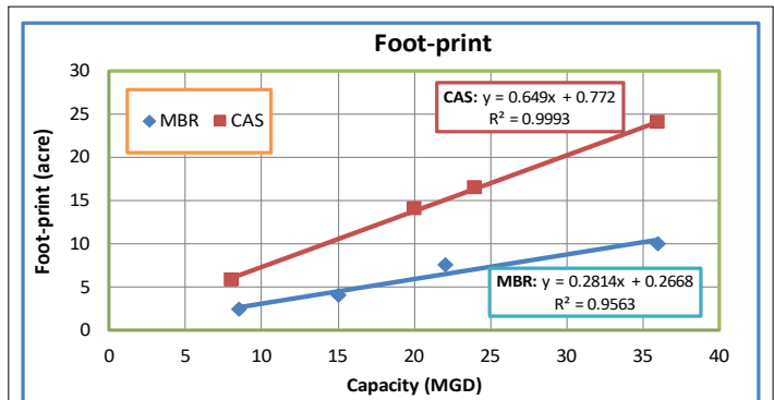
Figure 5: Variation of plant foot-print with plant capacity
